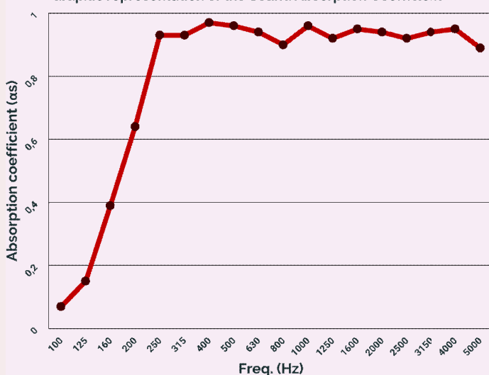
Graphic representation of the Sound Absorption Coefficient
